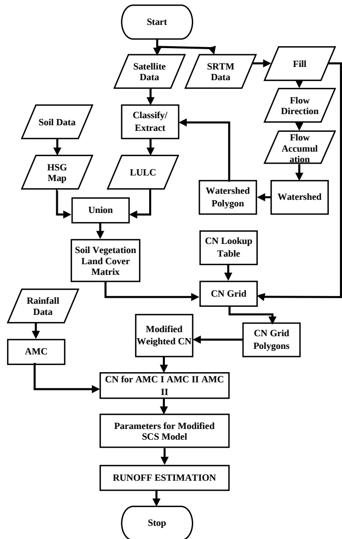
Figure 2: Schema for the Computation of Runoff in Kubanni Drainage Basin
