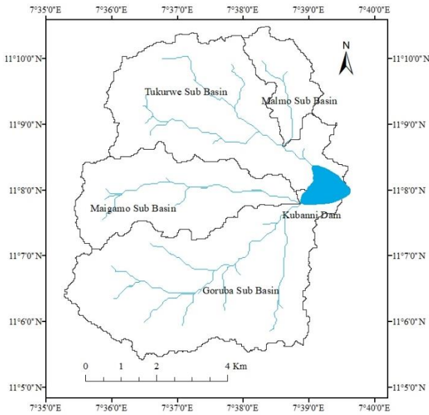
Figure 3: Kubanni basin model
