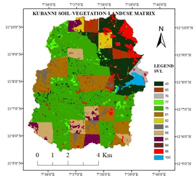
Figure 6: Soil-Vegetation-Land Use
