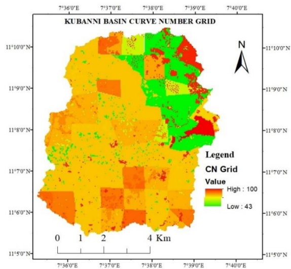
Figure 7: Kubanni Curve Number Grid Map
