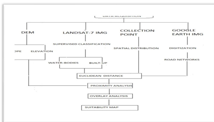
Figure 2: Summary of the Methodology
