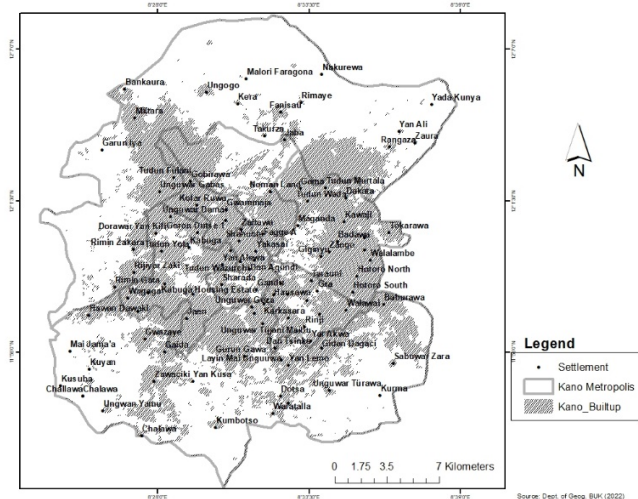
Figure 8A: Reclassified Built-Up suitability for landfill site in Kano Metropolis
