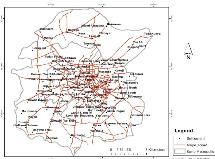
Figure 5B: Reclassified Road Suitability for Landfill Site in Kano Metropolis
