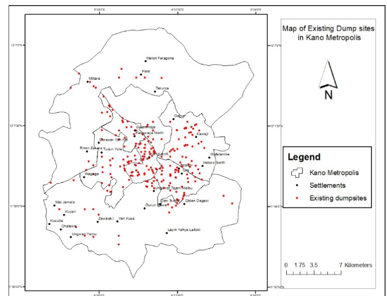
Figure 11A: Existing dumpsites constraint
