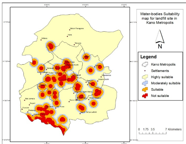
Figure 7B: Reclassified ponds suitability for landfill site in Kano Metropolis
