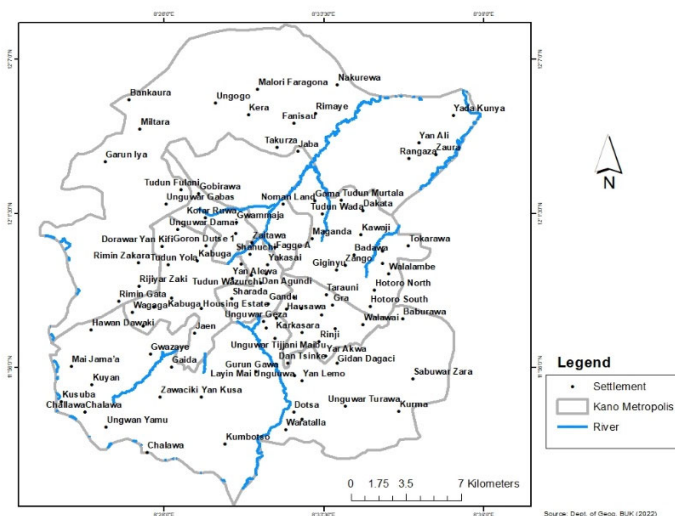
Figure 6 A: Surface Water (River) Constraint
