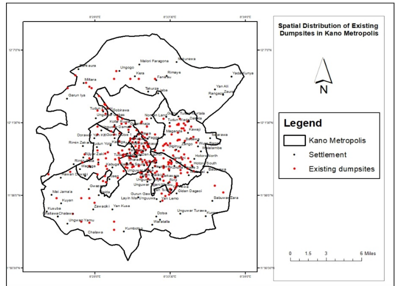
Figure 3: Distribution of Solid waste Dumpsites.
