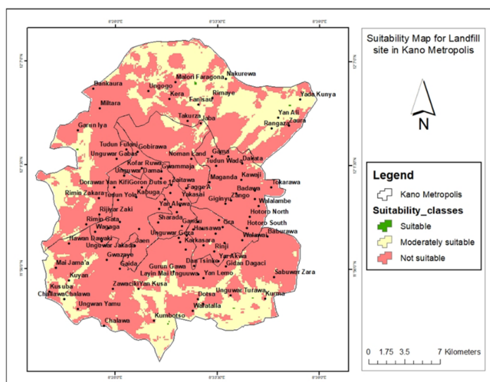
Figure 12: Suitability Areas for landfill site in Kano Metropolis.
