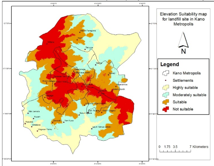
Figure 10B: Elevation constraint
