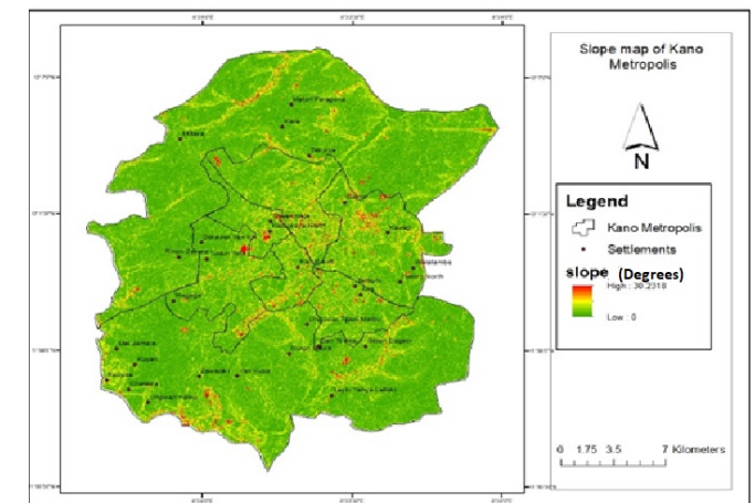
Figure 9A: Slope constraint
