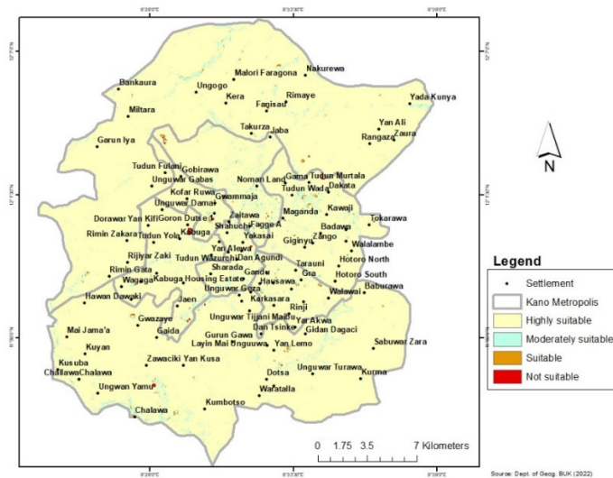
Figure 9B: Slope constraint
