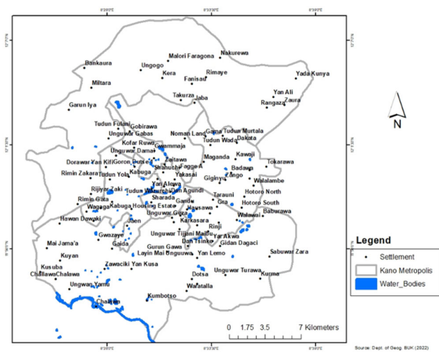
Figure 7A: Reclassified ponds suitability for landfill site in Kano Metropolis
