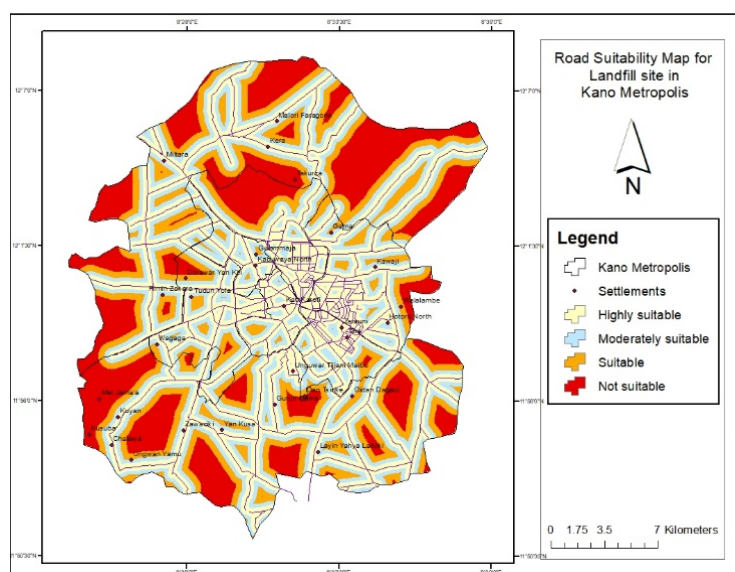
Figure 5A: Reclassified Road Suitability for Landfill Site in Kano Metropolis
