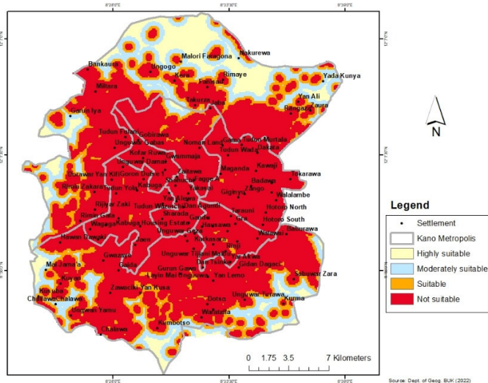
Figure 8B: Reclassified Built-Up suitability for landfill site in Kano Metropolis
