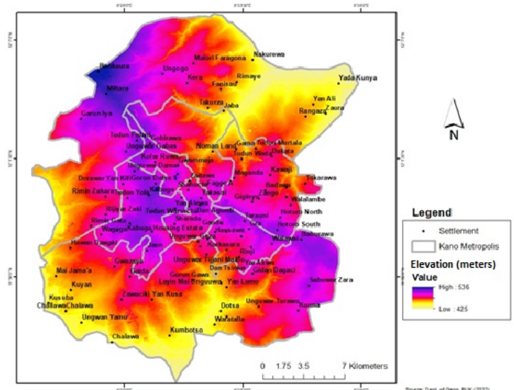
Figure 10A: Elevation constraint
