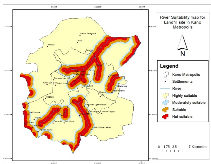
Figure 6 B: Surface water (River) Constraint
