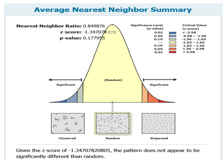
Figure 4: Average Nearest Neighbor Analysis
